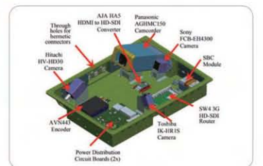
HDEV Payload Electronics Diagram
