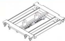
VGs Sub Frame (930-0023) Suspension frame for VGs subwoofers
